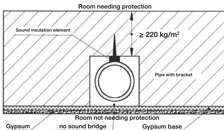
Traditional laying method (FIGURE 25)
