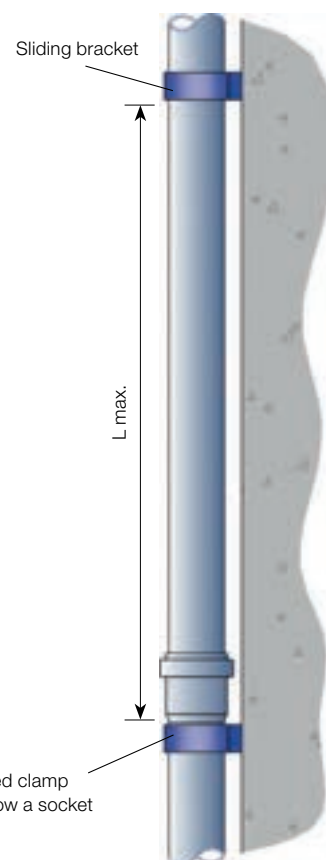
Vertical pipe routing (FIGURE 20)
